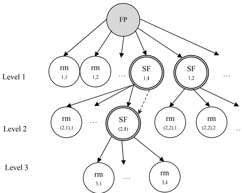
Fig. 1. Diagram of program modes for calculating the single-phase recipe
