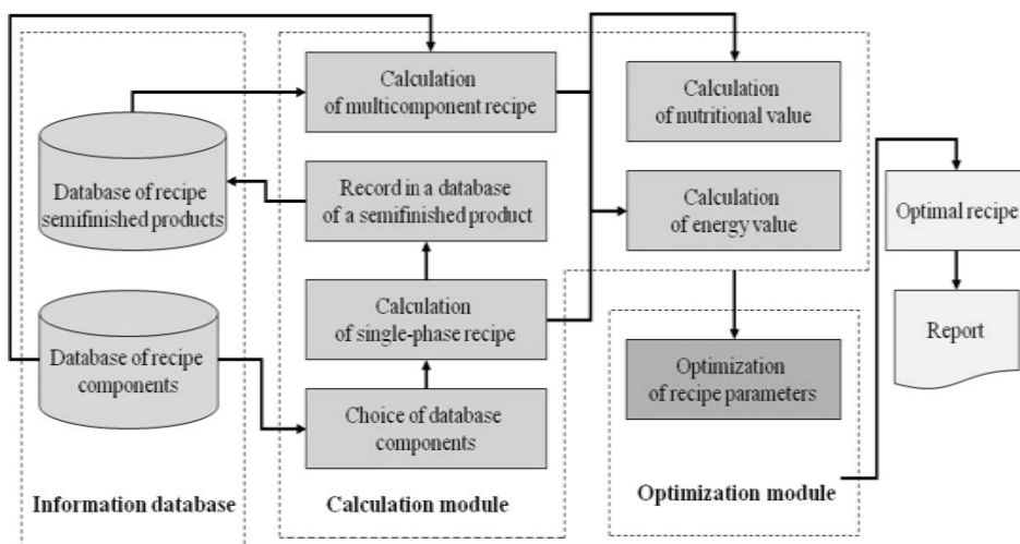
Fig. 3. Functional diagram of the system 'Multifaz'
